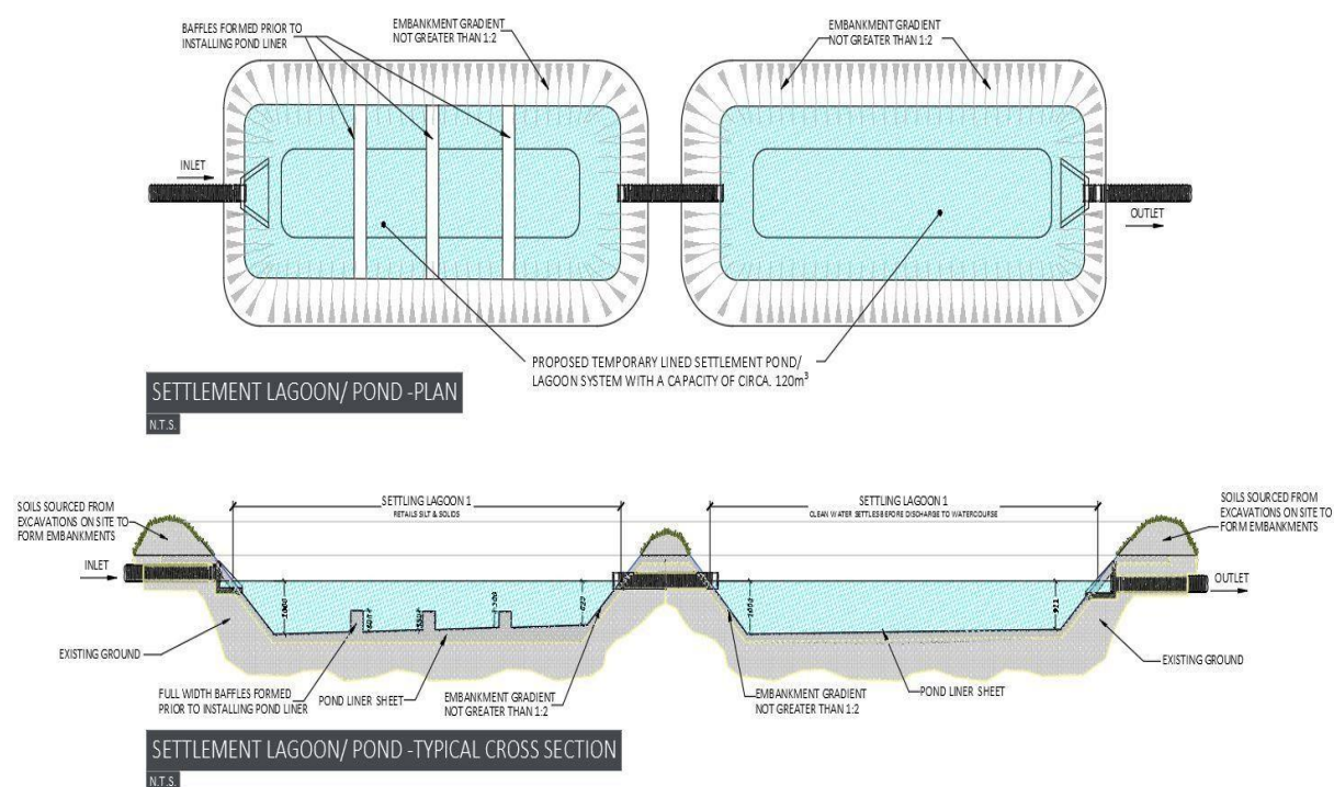
Figure 2.6.1- Example of a Typical Temporary Settlement Lagoon/ Pond
